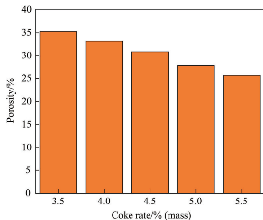
Fig. 6. Effect of coke rate on porosity of sinter.
