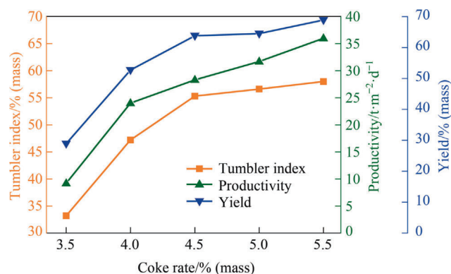
Fig. 10. Effect of coke rate on sinter indexes.
