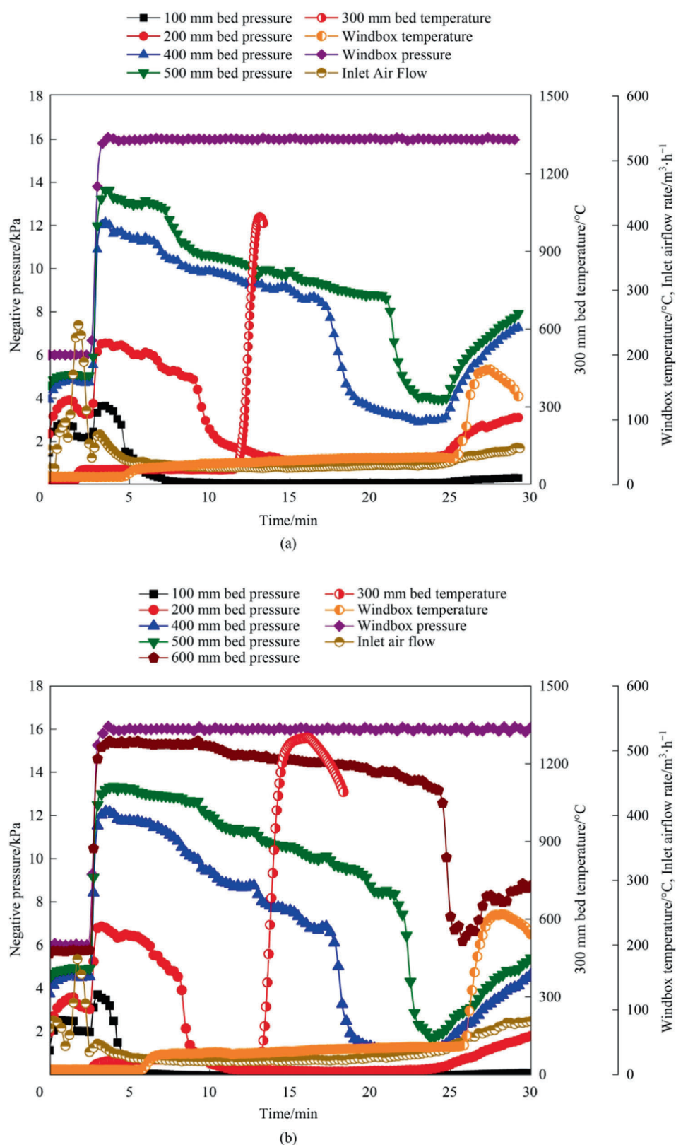
Fig. 4. In situ sintering bed negative pressures and temperature, windbox negative pressure and temperature, and inlet airflow rate at (a) 3.5% (mass) coke rate and (b) 5.5% (mass) coke rate.
